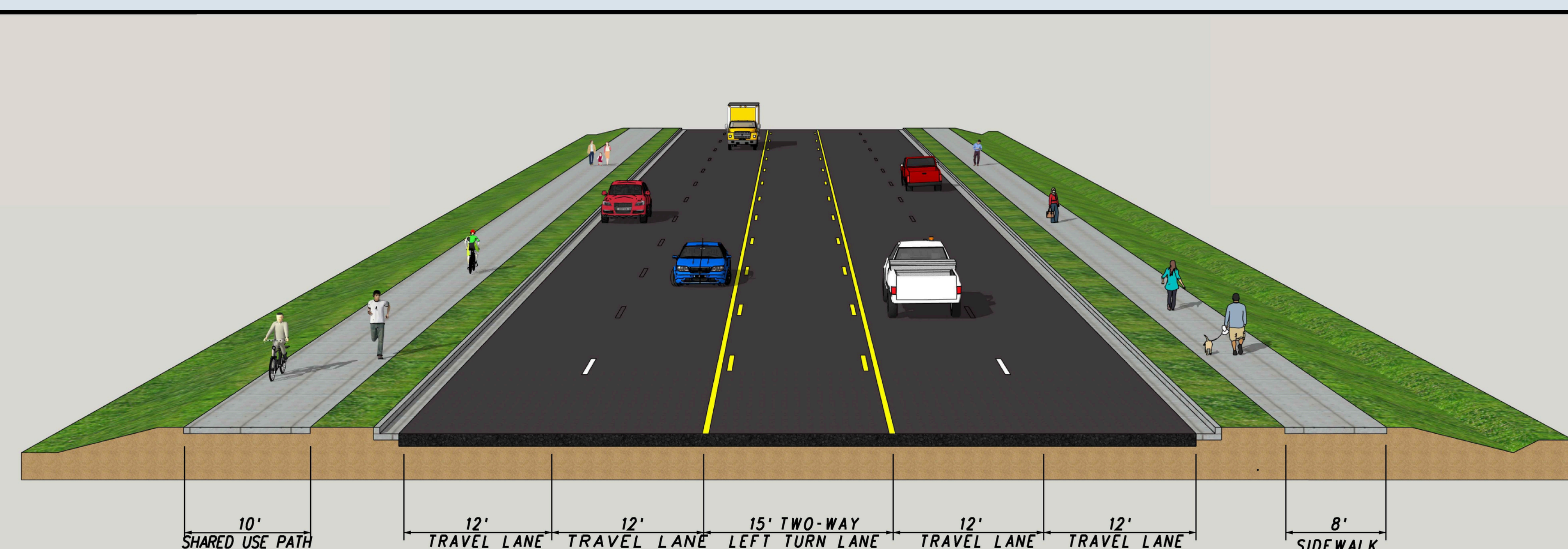
MILES JAMISON ROAD 5 LANE CURB & GUTTER SECTION
